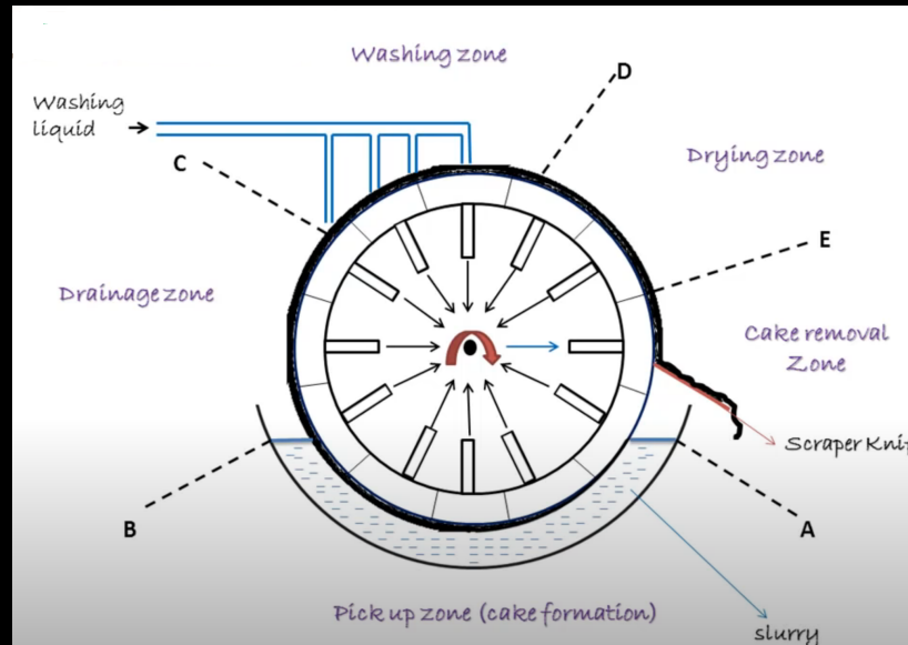
Figure 5: Schematic of a rotary vacuum filter.(Image source: Ahmed Abdel0Moneim Ali, Cairo University)
