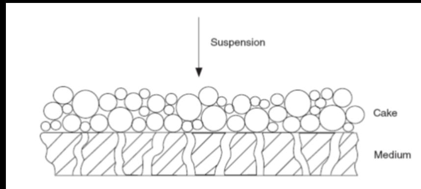
Figure 1: Schematic of cake filtration.
