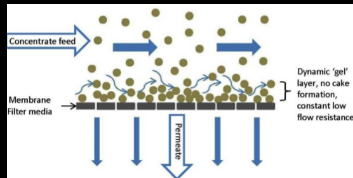
Figure 3: Schematic of cross flow filtration
