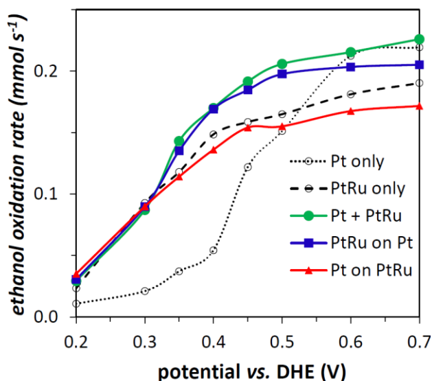
Figure 6. Ethanol consumption rate vs. potential for the oxidation of 0.100 M ethanol (0.2 mL min -1 and 80 °C) at Pt (···), PtRu (- - -), Pt + PtRu (●), Pt on PtRu (▲) and PtRu on Pt (■) anodes.
